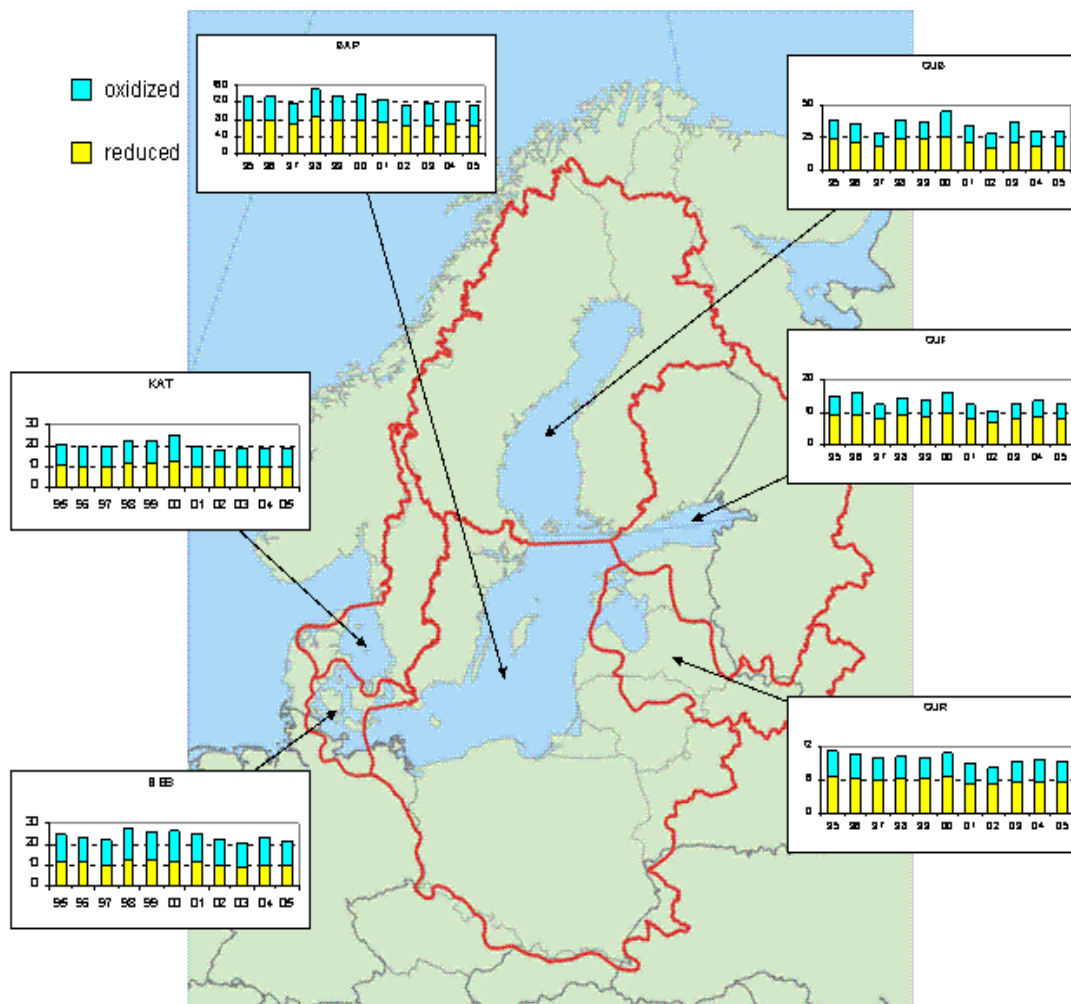
Figure 2. Atmospheric deposition of oxidized, reduced and total nitrogen to six sub-basins of the Baltic Sea for the period 1995 - 2005. Units: ktonnes N/year. Note: the scales for the sea regions are different!
