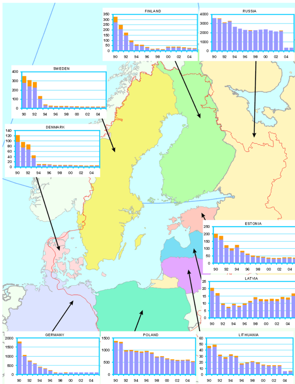
Figure 4: Map of lead emissions of HELCOM Contracting Parties (CP) to air as totals in tonnes/year for the period 1990-2005. Red sections of the bars identify the fraction of emission deposited to the Baltic Sea. ( The emission data of the CP refer to the total area of the CP except for Russian Federation, for which emissions from the territory of Russian Federation within the EMEP domain is used ).
