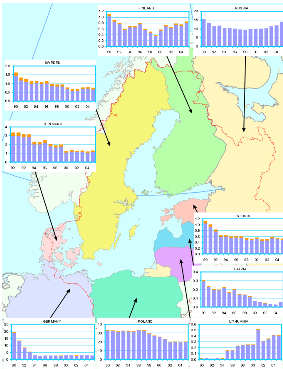
Figure 3: Map of mercury emissions of HELCOM Contracting Parties (CP) to air as totals in tonnes/year for the period 1990-2005. Red sections of the bars identify the fraction of emission deposited to the Baltic Sea. ( The emission data of the CP refer to the total area of the CP except for Russian Federation, for which emissions from the territory of Russian Federation within the EMEP domain is used ).
