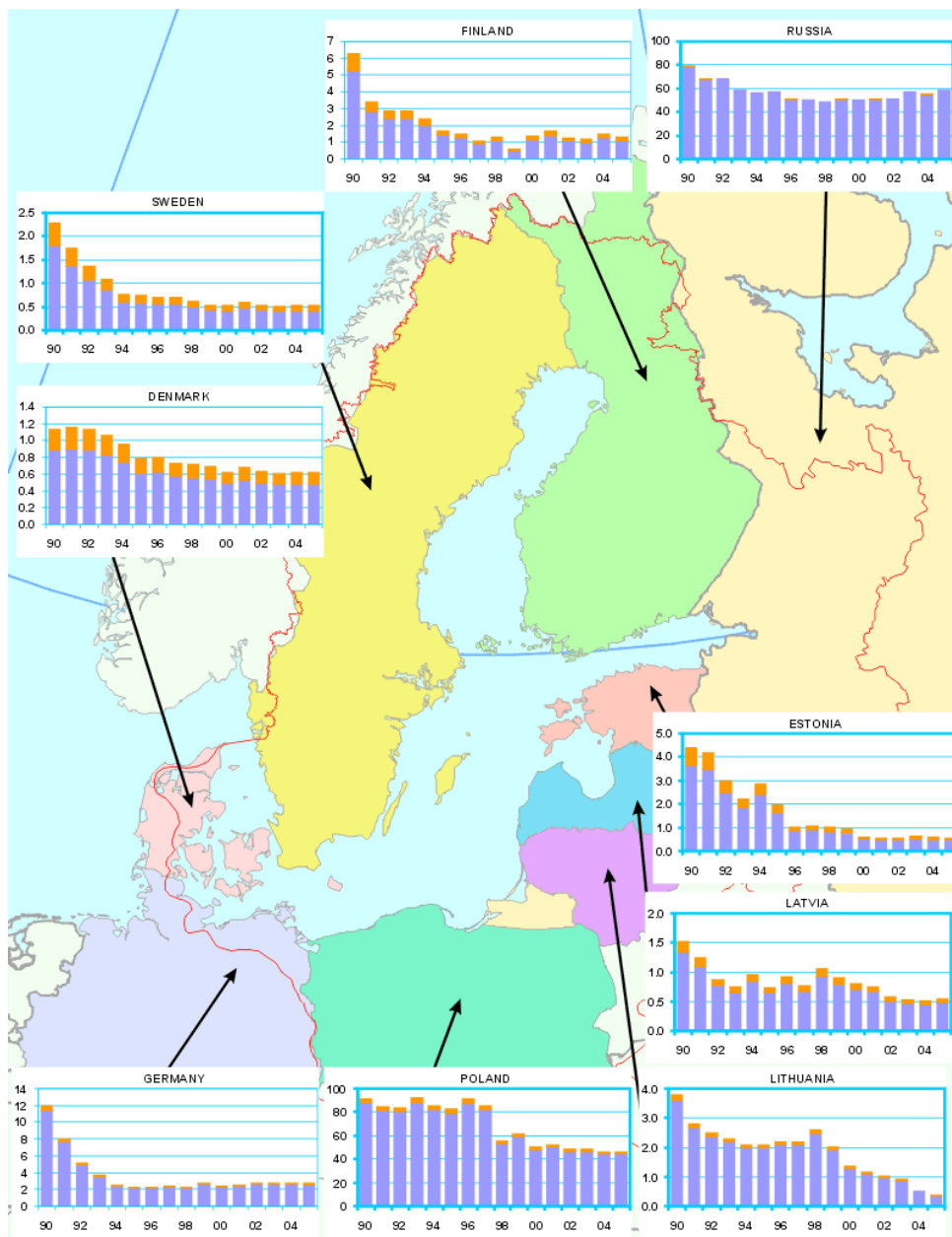
Figure 2: Map of cadmium emissions of HELCOM Contracting Parties (CP) to air as totals in tonnes/year for the period 1990-2005. Red sections of the bars identify the fraction of emission deposited to the Baltic Sea. ( The emission data of the CP refer to the total area of the CP except for Russian Federation, for which emissions from the territory of Russian Federation within the EMEP domain is used ).
