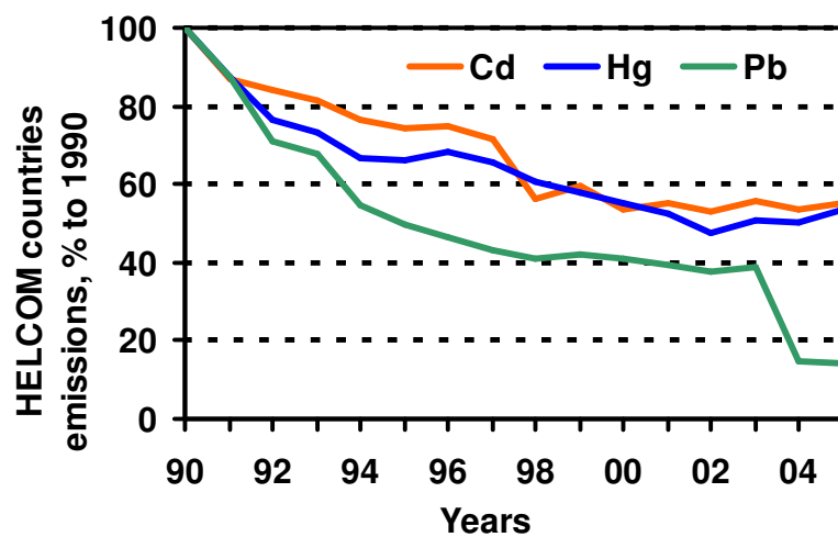
Figure 1. Total annual emissions of cadmium, mercury, and lead to air from HELCOM countries in period 1990-2005 (% of 1990).
