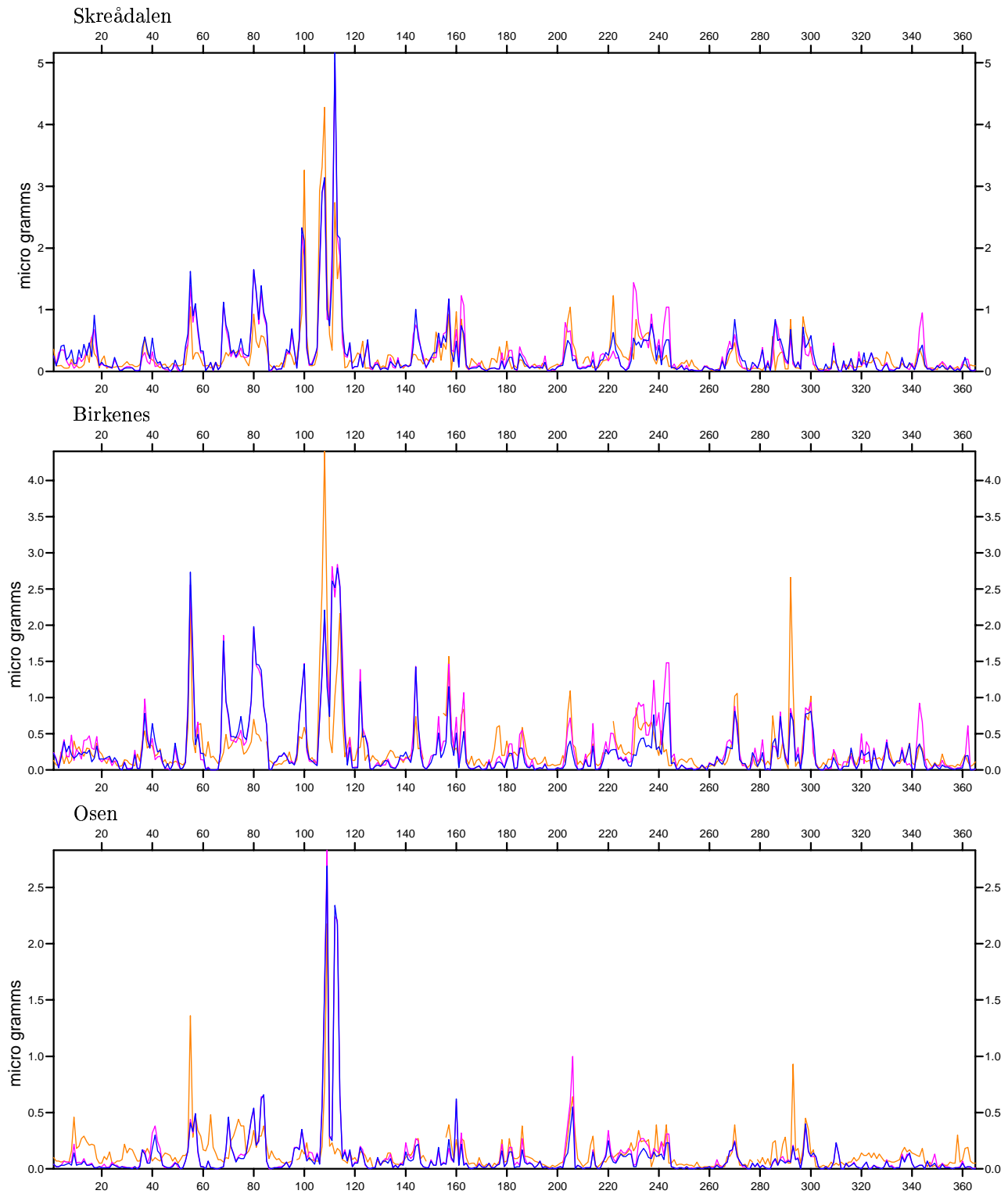
Figure 6.6: Measured (yellow) concentrations of total nitrate in \mu\text{g}(\text{N})\text{cm}^{-3} versus calculated, (red) with \text{NaNO}_3 , (blue) without \text{NaNO}_3 . Results for 1996.
