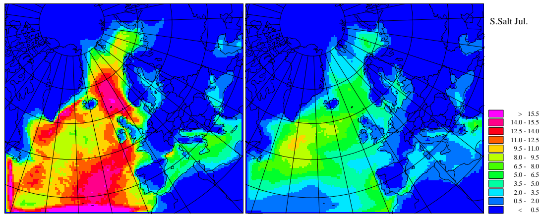
Figure 6.3: Monthly averaged surface concentrations of sea salt in \mu\text{g}(\text{Na})\text{cm}^{-3} for (left) January and (right) July, 1996.
