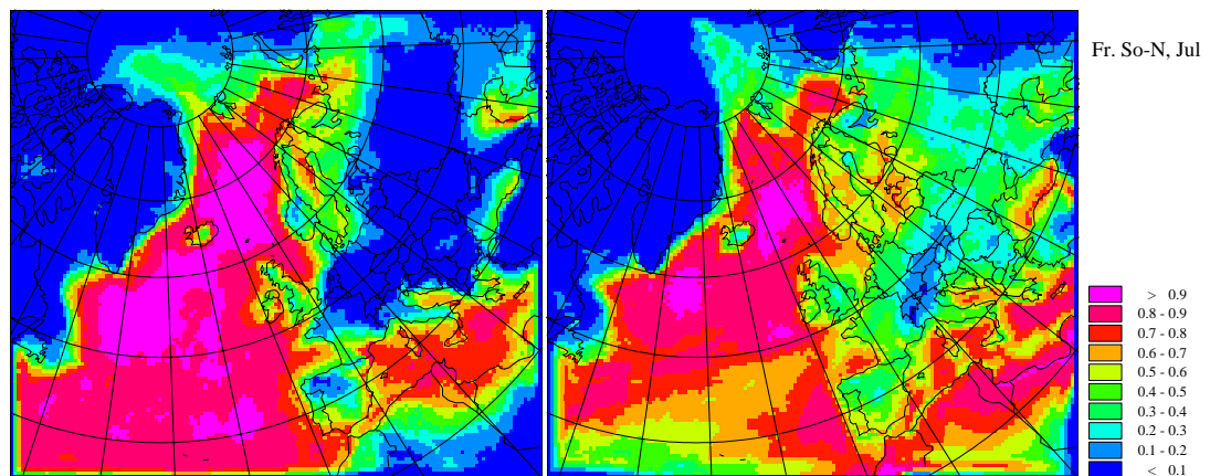
Figure 6.4: Monthly averaged fraction of total nitrate in the form of sodium nitrate in (left) January and (right) July, 1996.
