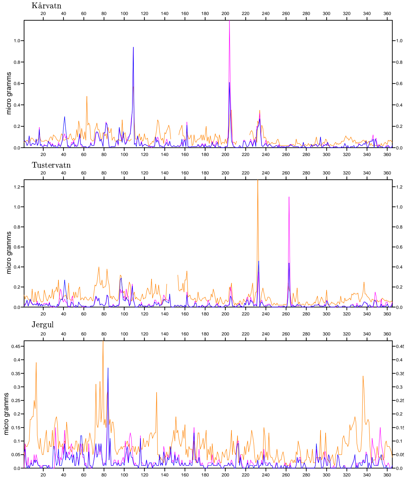
Figure 6.7: Measured (yellow) concentrations of total nitrate in \mu\text{g}(\text{N})\text{cm}^{-3} versus calculated, (red) with \text{NaNO}_3 , (blue) without \text{NaNO}_3 . Results for 1996.
