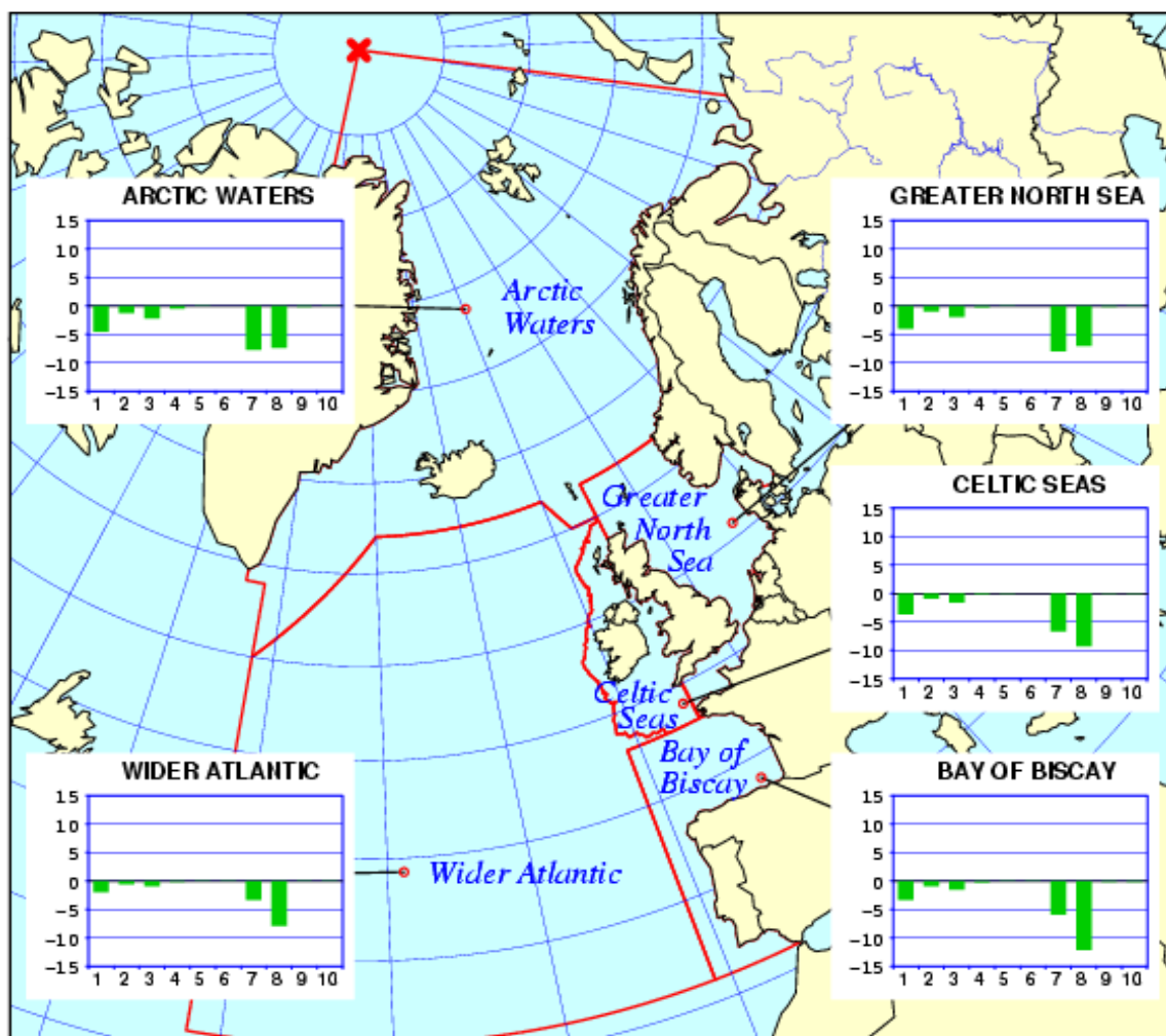
Figure 38. Reduction of annual oxidized nitrogen deposition (in percent of initial deposition) due to 25 % reduction of \text{NO}_x emissions in each of 10 SNAP sectors in the year 2000. Green color denotes reduction of deposition and red color denotes increased deposition from given sector.
