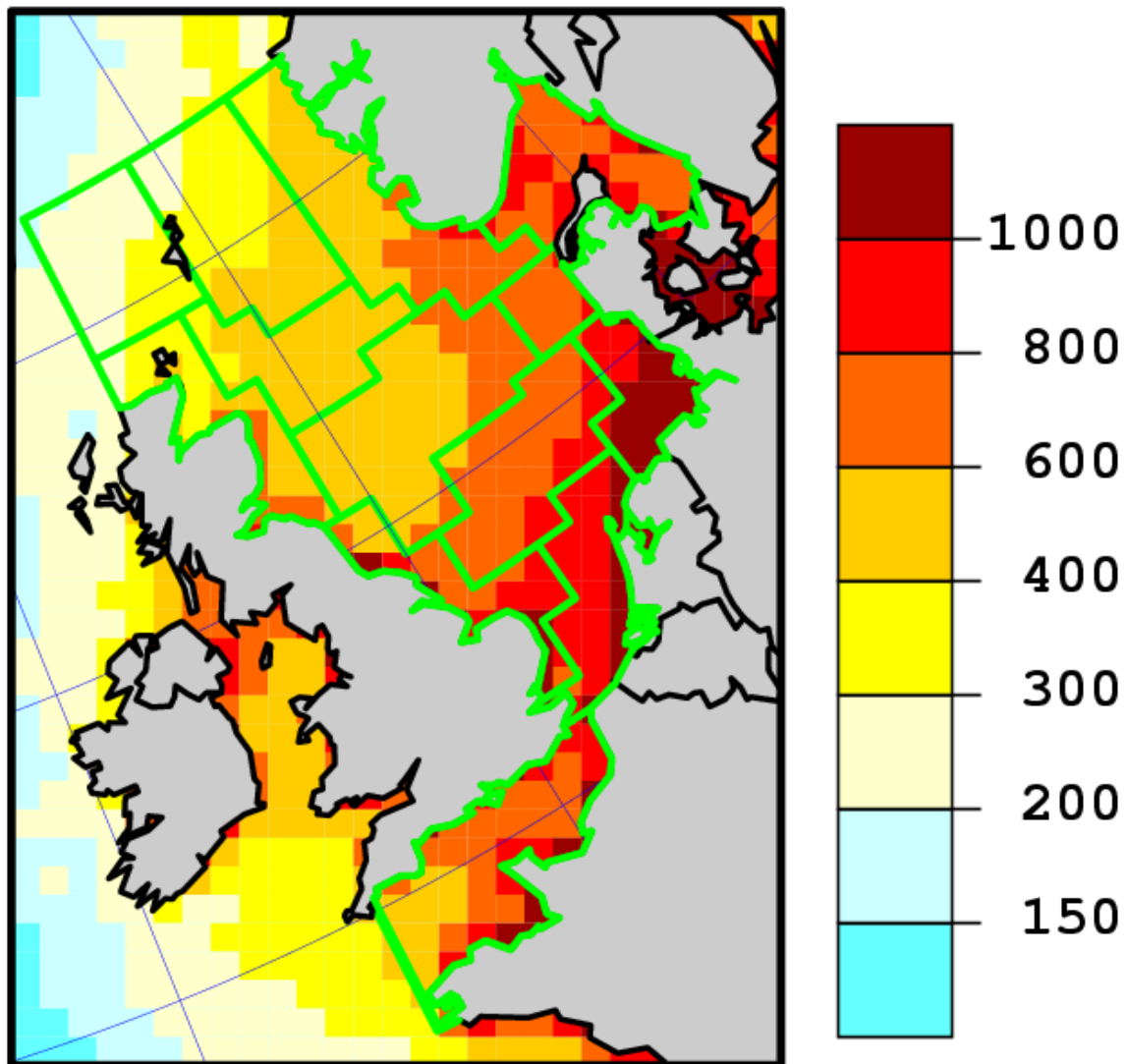
Figure 18. Map of modelled total annual nitrogen (oxidized and reduced) deposition in 13 sub-regions of OSPAR Region II (Greater North Sea) in 2001. Unit: mg N m -2 .
