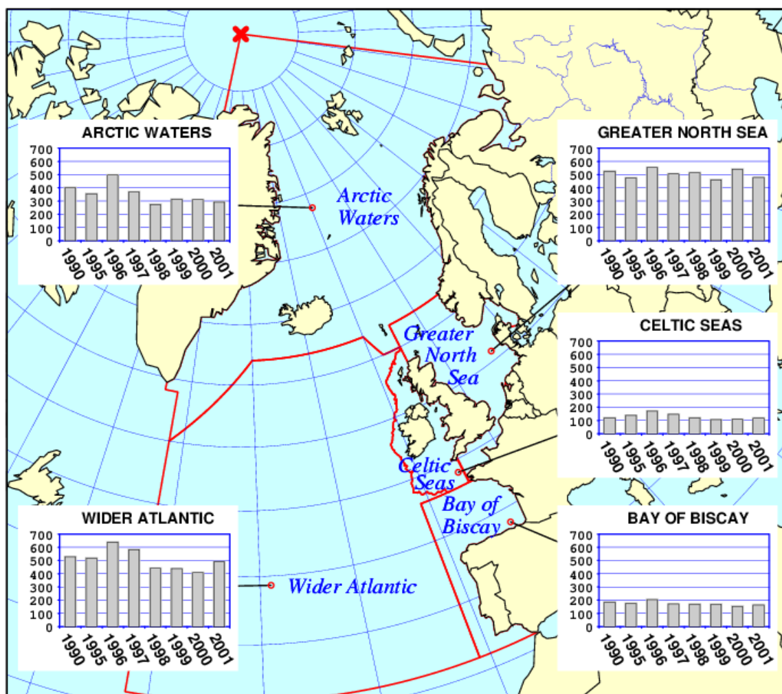
Figure 21. Map with time series of modelled total annual nitrogen (oxidized + reduced) deposition in the five main OSPAR regions. Unit: \text{kt N a}^{-1} .
