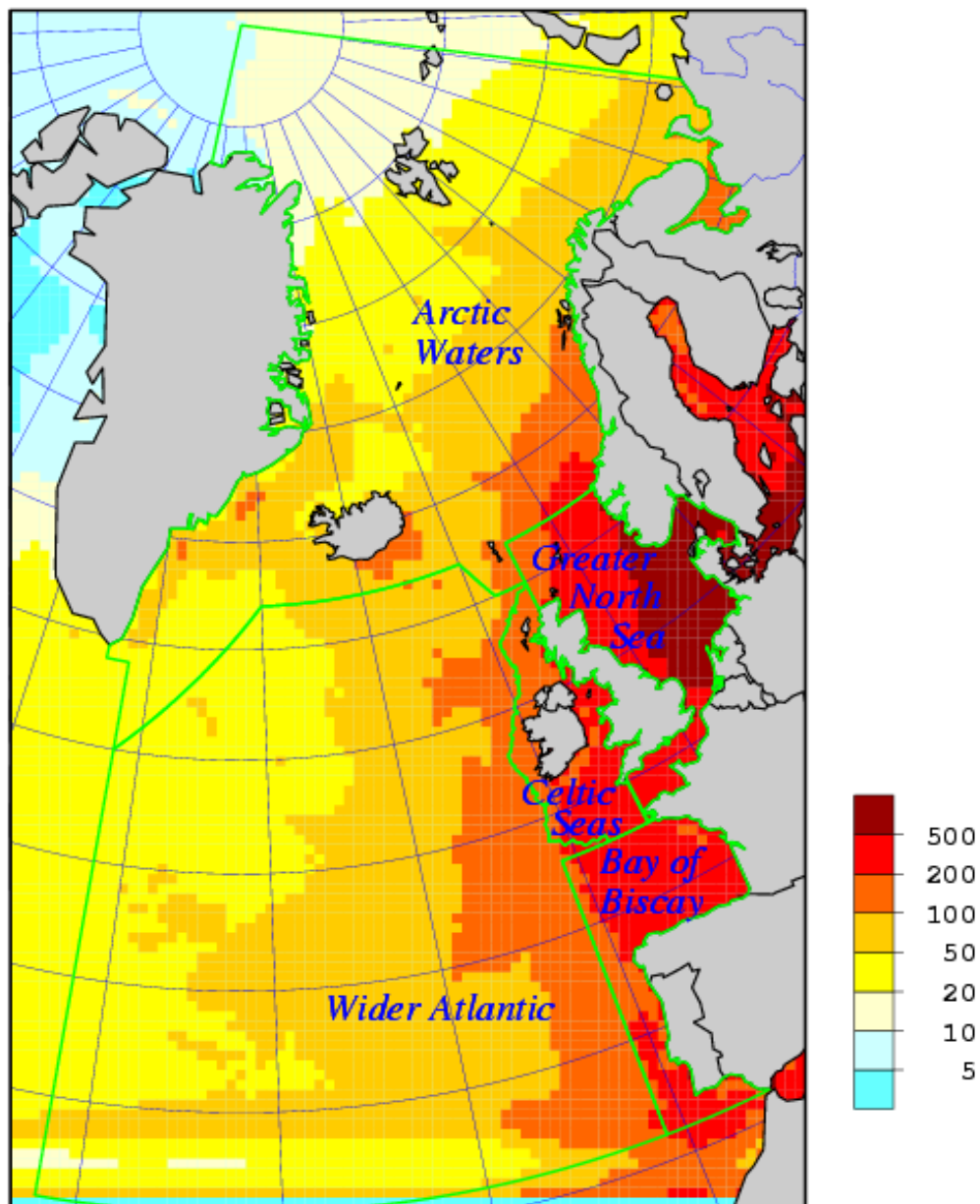
Figure 6. Map of modelled annual oxidized nitrogen deposition in the five main OSPAR regions in 1990. Unit: mg N m -2 .
