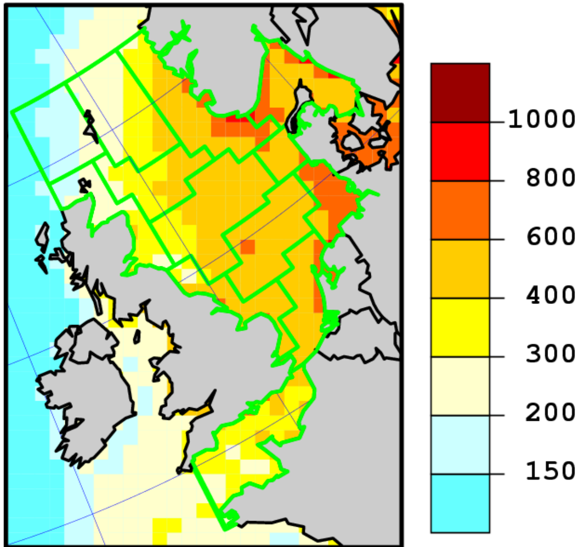
Figure 13. Map of modelled annual oxidized nitrogen deposition in 13 sub-regions of OSPAR Region II (Greater North Sea) in 1990. Unit: \text{mg N m}^{-2} .
